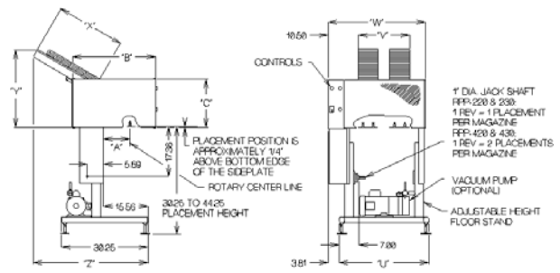
Parallel Jackshaft with Stand
