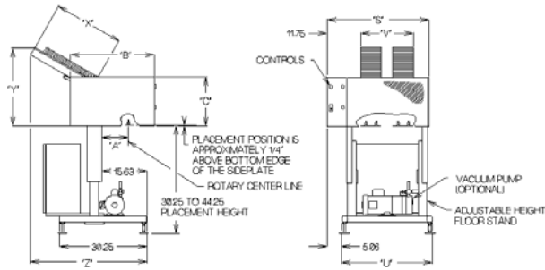
Servo Drive with Stand
